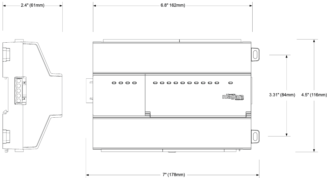
Figure 2: IO-R-34 dimensions
