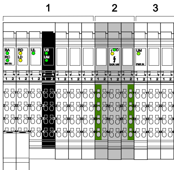
Fig. 5: Switching of 230 V within a 24 V area
