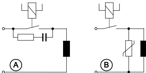
Fig. 7: Contact protective circuit (A), -load protective circuit (B)
