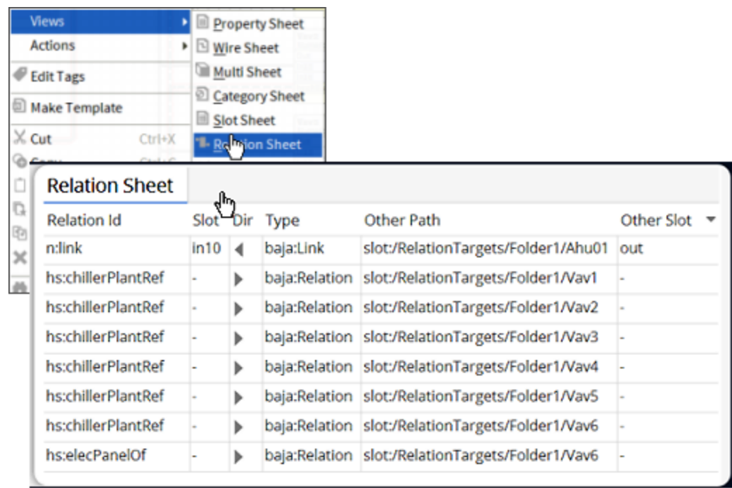
Figure 3. Relation Sheet view shows relations and links
