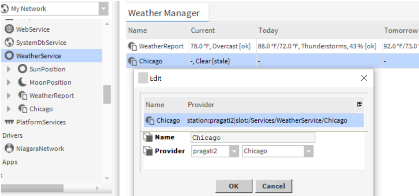
Figure 26. Edit dialog of added WeatherReport shows FoxWeatherProvider selections
