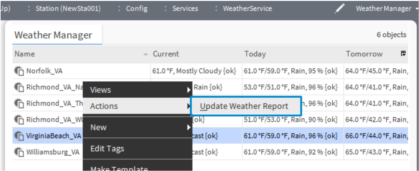
Figure 9. WeatherReport action
