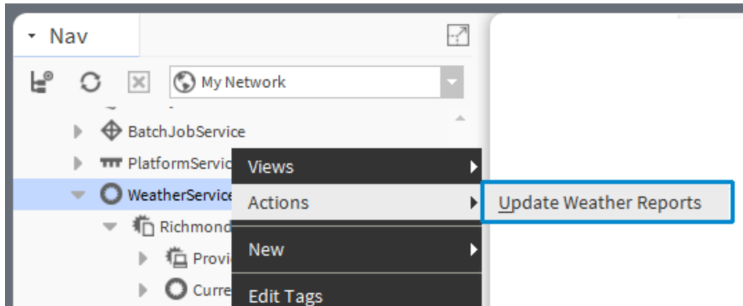
Figure 7. WeatherService action
