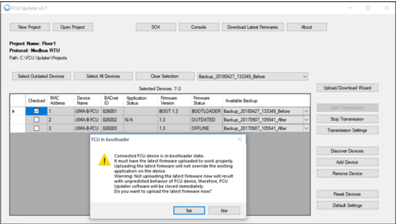
Figure 52. FCU Updater recognizes a bootloader state in one controller
