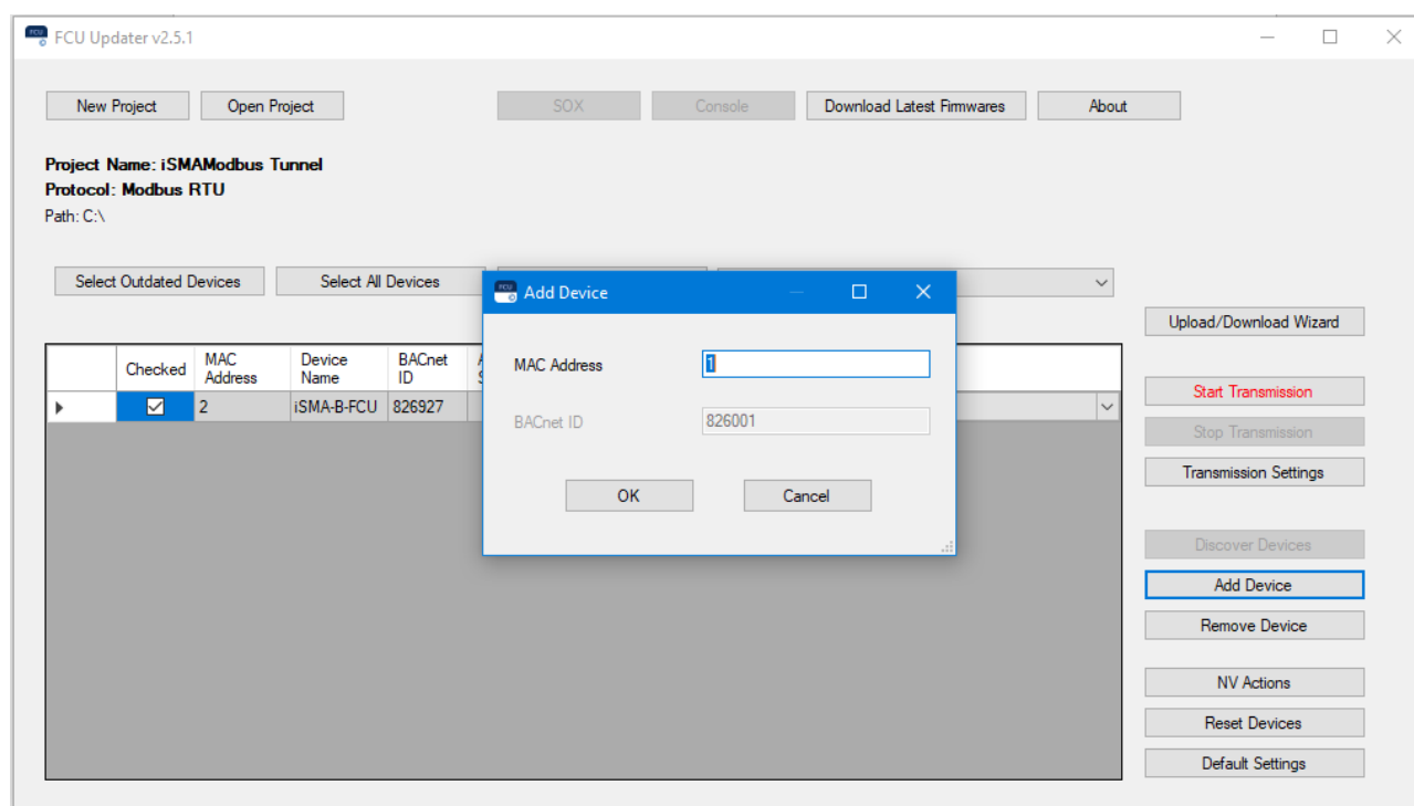
Figure 36. Add Device dialog window
