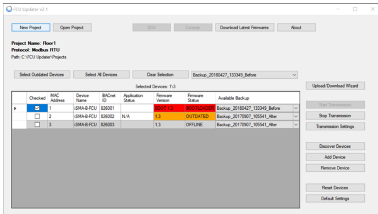
Figure 51. One of controllers in a bootloader state
