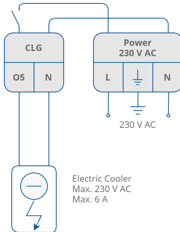
Figure 42. Configuration of the 2-stage electrical cooler and the 2-stage of cooling activating CFG DIP switch
