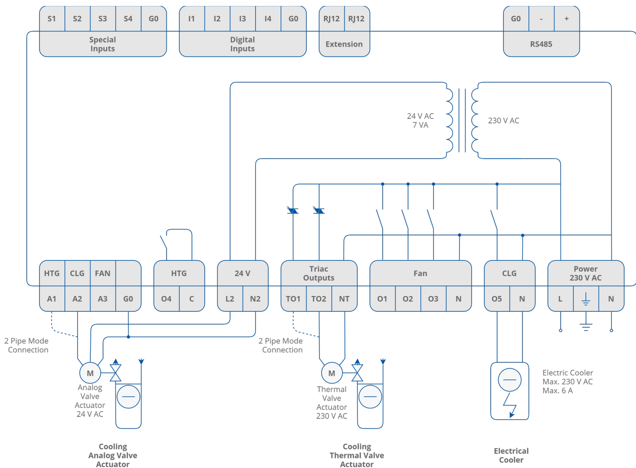
Figure 36. Example connections of FCU-HH cooling devices
