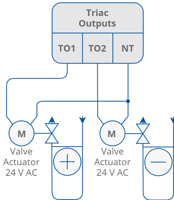
Figure 22. Connection of thermal valve actuator to triac outputs (FCU-HL and FCU-LL)
