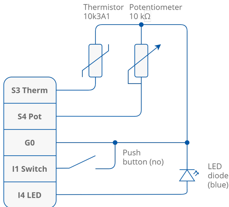
Figure 16. Diagram of internal connections of the simple panel
