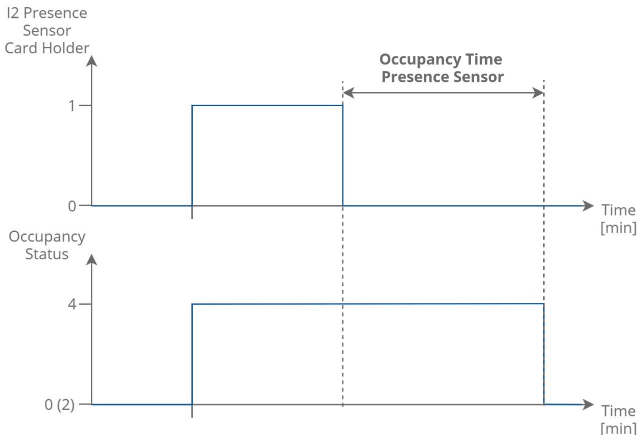
Figure 6. Presence sensor or card holder function time
