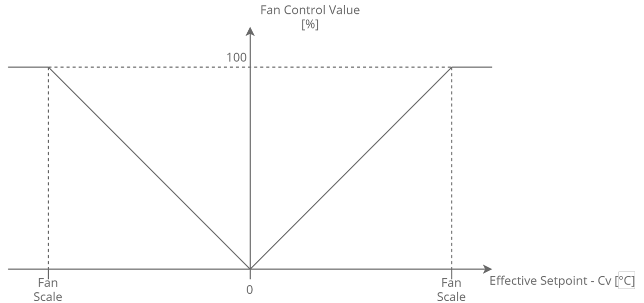
Figure 49. Fan control value conversion chart
