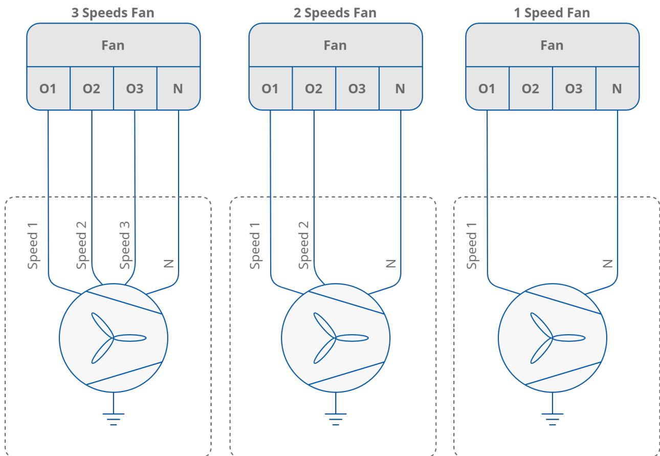
Figure 11. Fan connections
