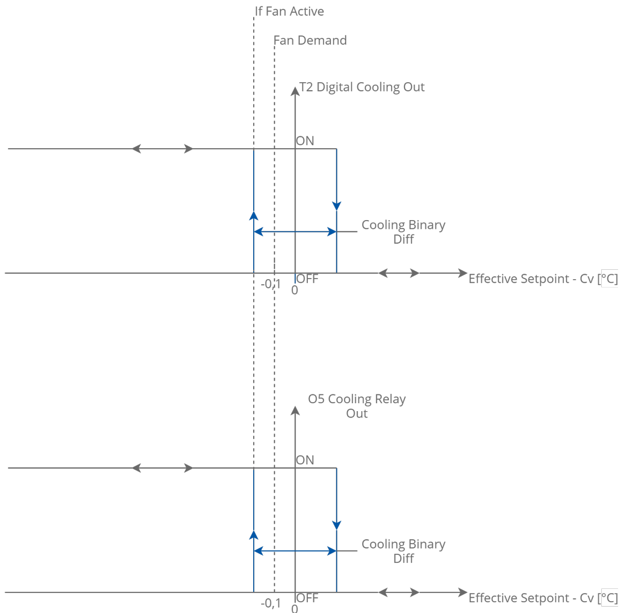
Figure 38. 1-stage cooling digital control mode
