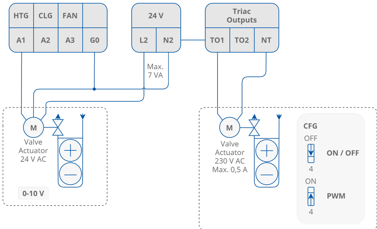
Figure 24. Connection of heating/cooling valve actuators in 2-pipe mode
