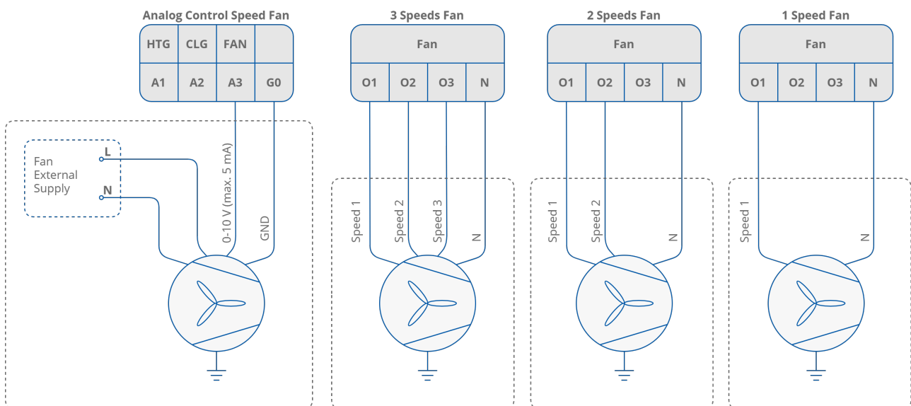
Figure 48. Fan motor connection according to the fan control mode
