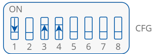
Figure 45. CFG DIP switch configuration for analog control mode
