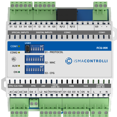
Figure 1. FCU-HH controller
