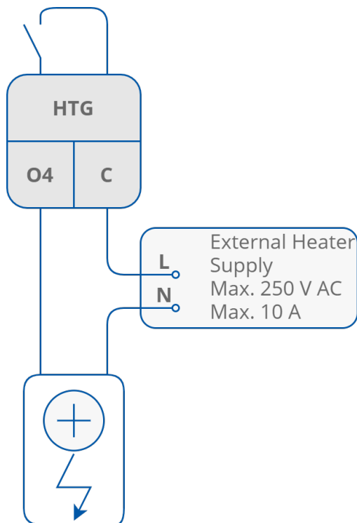
Figure 31. 2-stage electrical heater connection and heating 2nd stage of heating activated CFG DIP switch configuration
