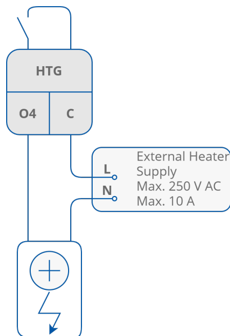
Figure 12. Electrical heater connections
