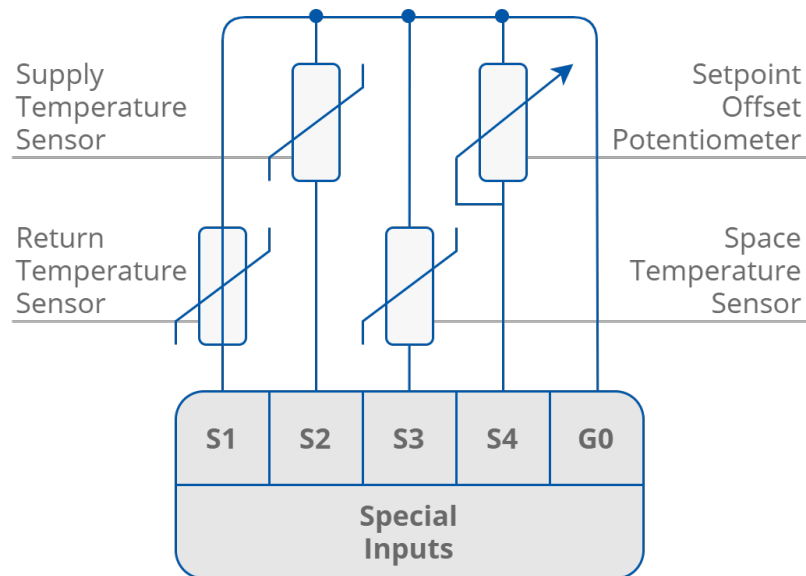
Figure 7. Special inputs connection
