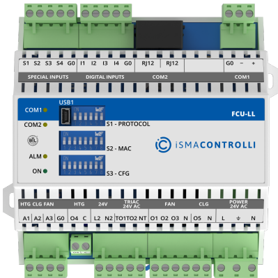
Figure 3. FCU-LL controller
