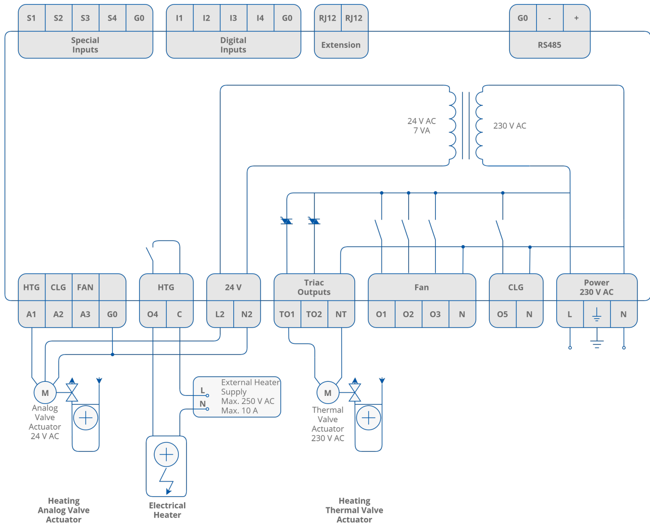
Figure 25. Example connection of FCU-HH heating devices
