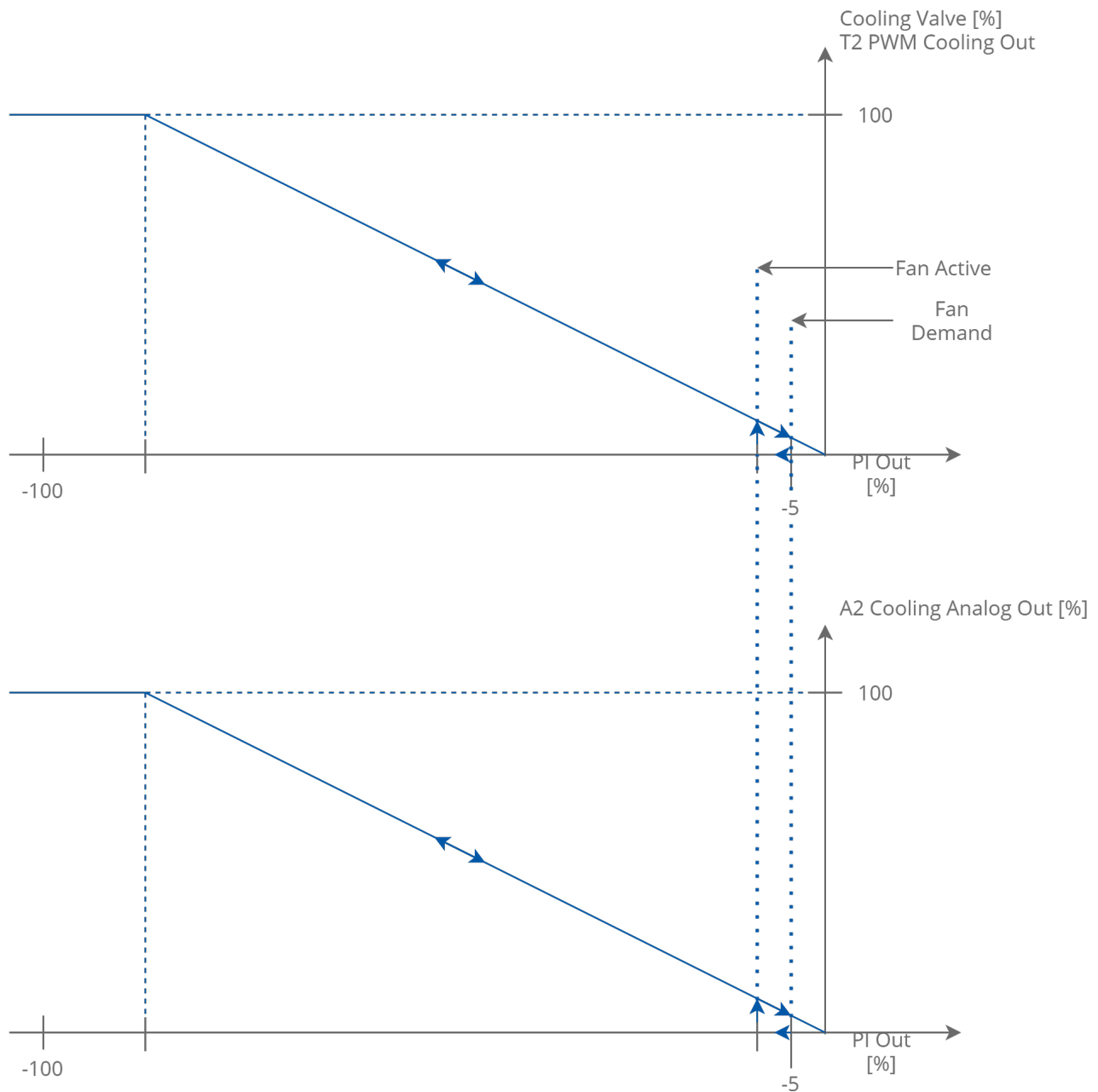
Figure 40. 1-stage cooling analog control mode
