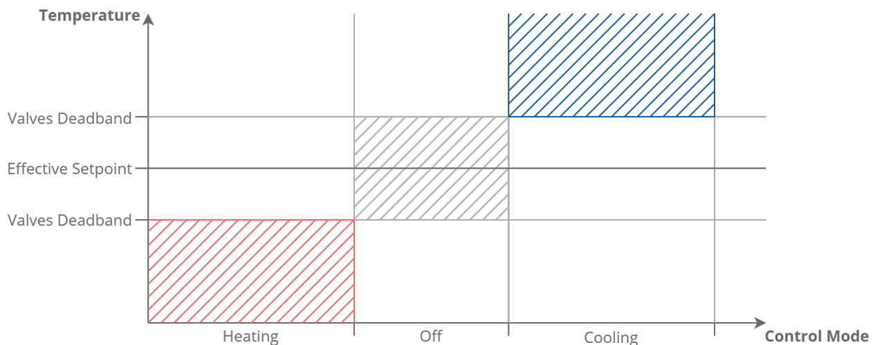
Figure 47. Valve dead band operation chart
