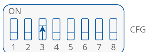
Figure 41. 2-stage cooling DIP switch configuration
