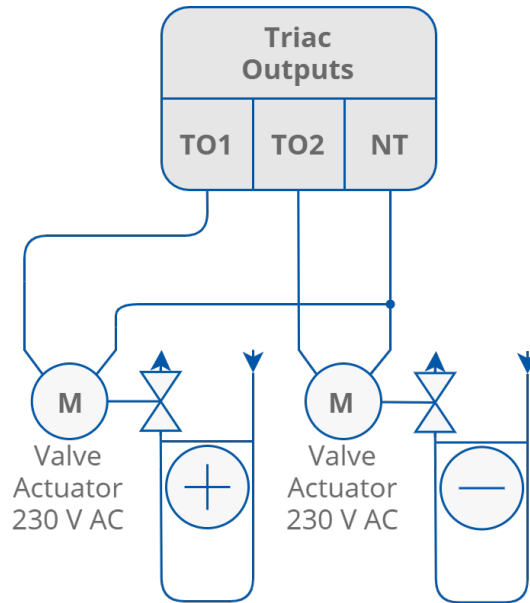
Figure 9. Triac outputs connection
