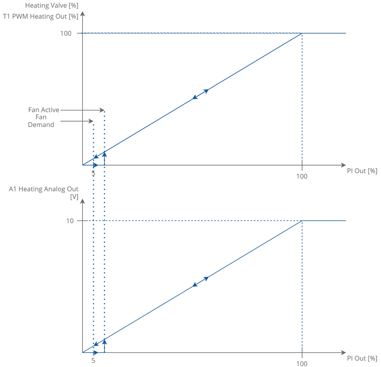
Figure 29. 1-stage heating analog control mode
