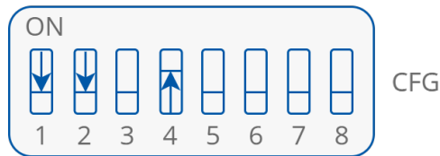
Figure 28. CFG DIP switch configuration for analog control mode
