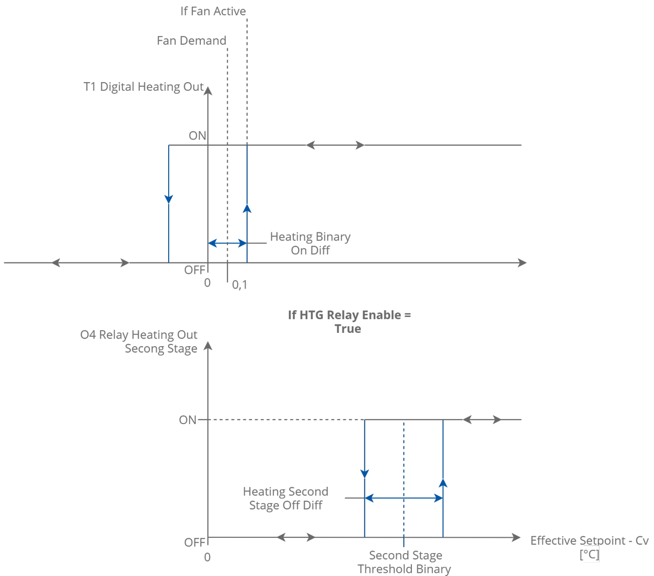
Figure 33. 2-stage heating digital control mode
