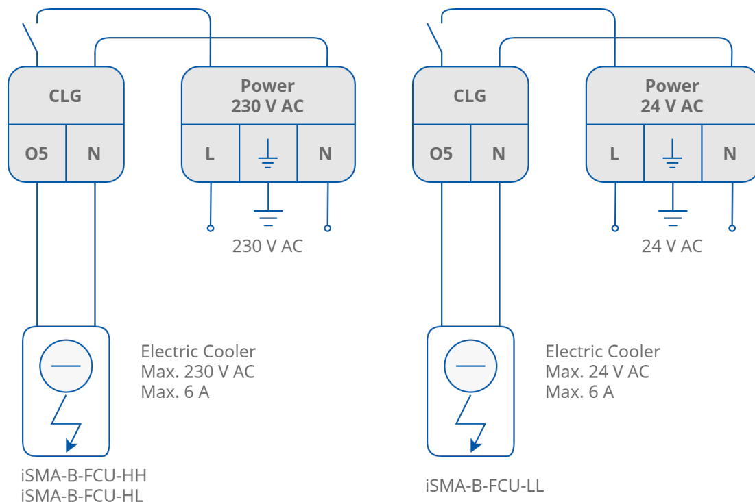
Figure 13. Electrical cooler connection
