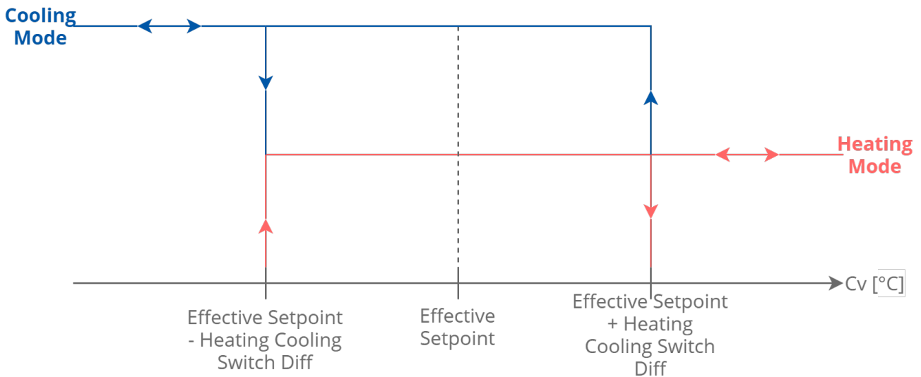
Figure 4. Switching between heating/cooling chart
