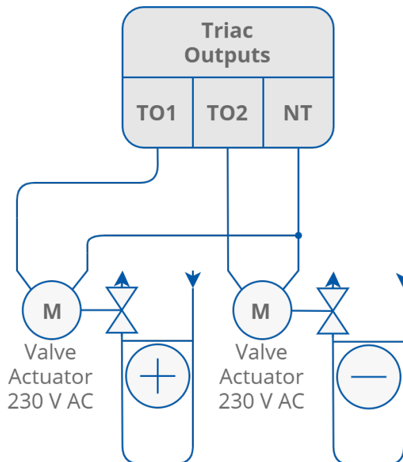
Figure 21. Connection of thermal valve actuator to triac outputs (FCU-HH)
