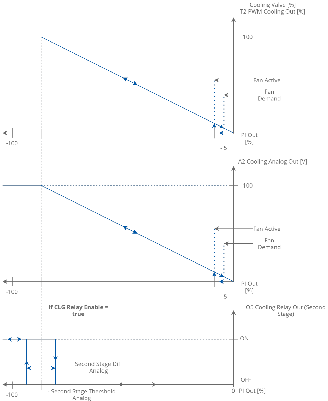
Figure 46. 2-stage cooling analog control mode
