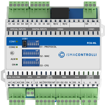
Figure 2. FCU-HL controller
