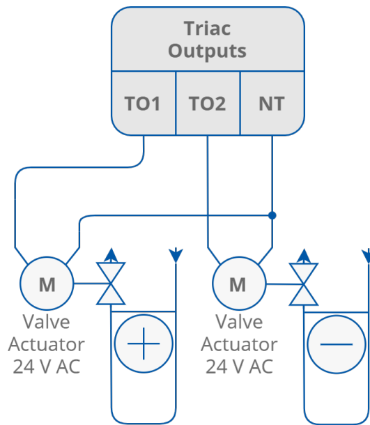
Figure 10. Connection of thermal valve actuators to triac outputs
