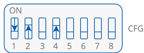
Figure 34. CFG DIP switch configuration for analog control mode
