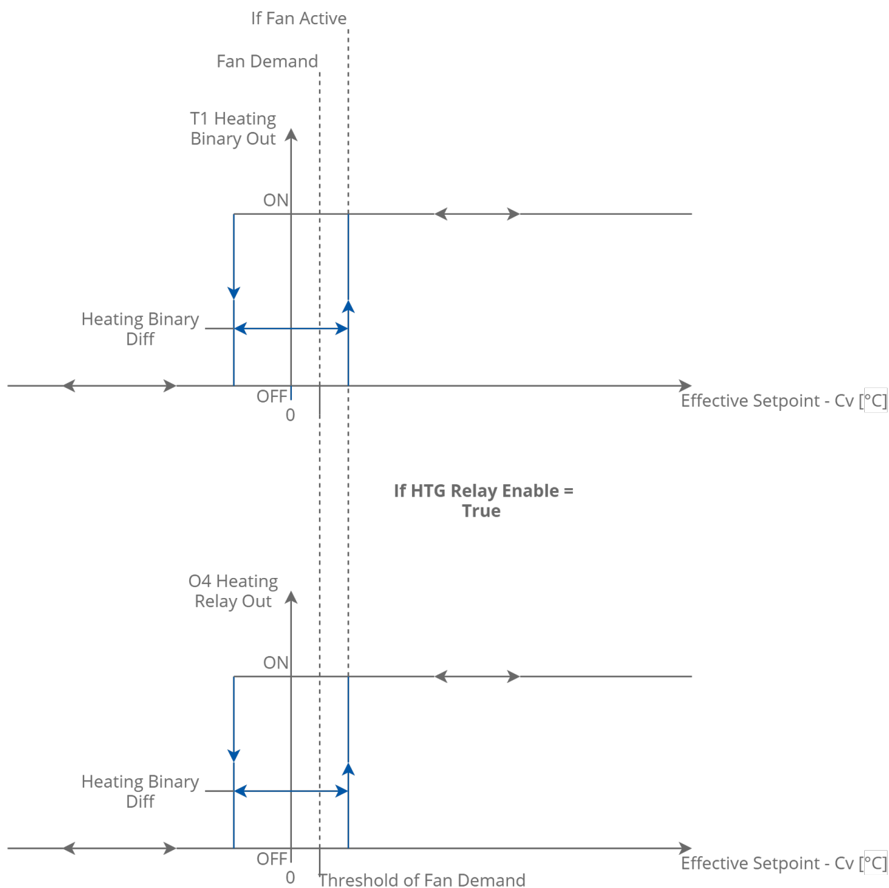
Figure 27. 1-stage heating digital control mode
