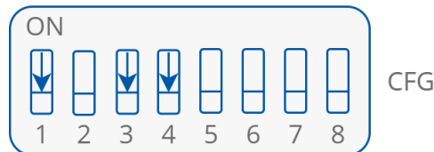
Figure 37. CFG DIP switch configuration for digital control mode
