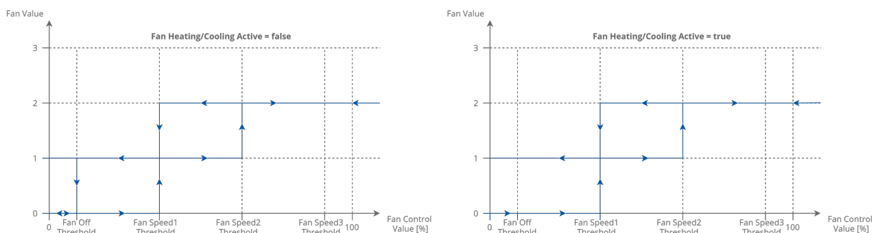
Figure 52. Fan 2-speed type control algorithm
