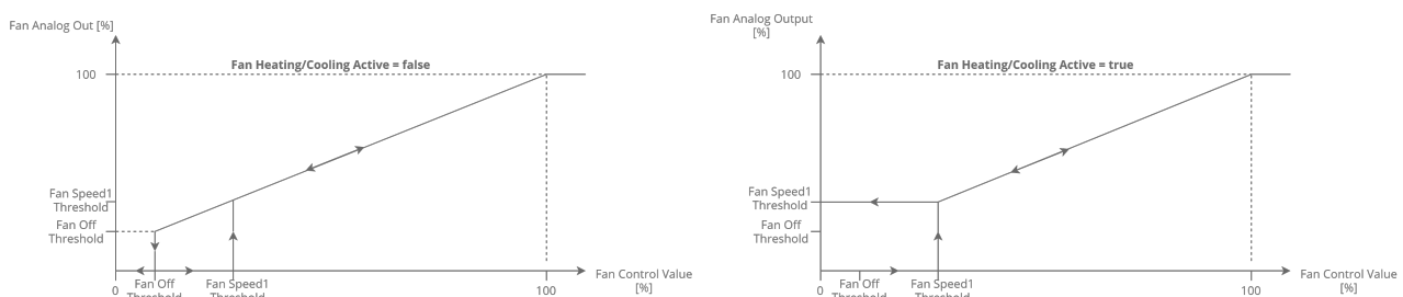
Figure 50. Fan analog type control algorithm
