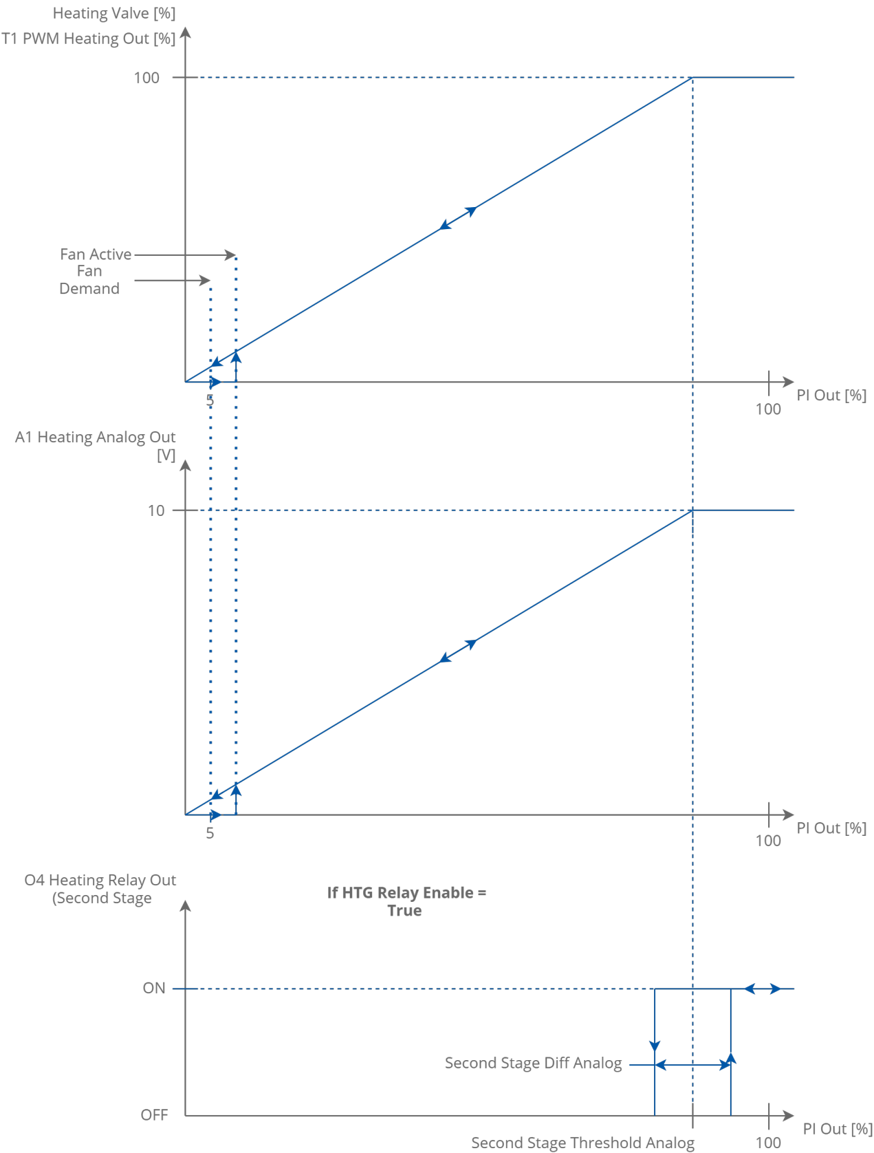
Figure 35. 2-stage heating analog control mode
