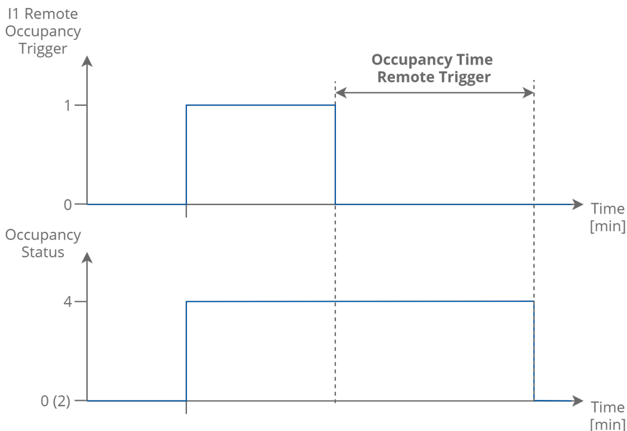
Figure 5. Occupancy trigger time function
