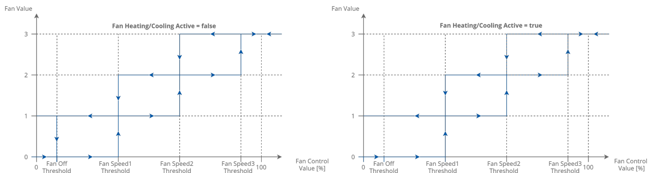
Figure 53. Fan 3-speed type control algorithm
