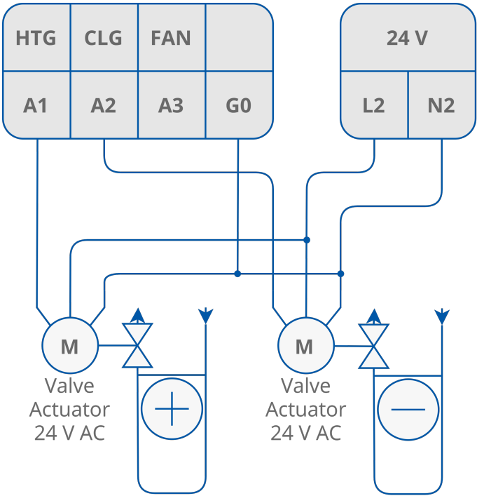
Figure 14. Connection of analog valve actuators
