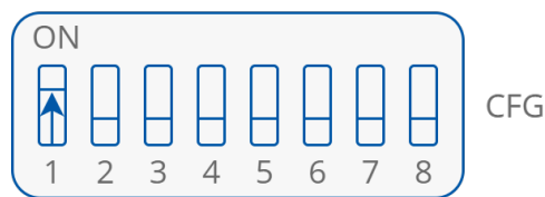
Figure 23. 2-pipe DIP switch configuration
