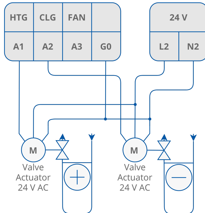
Figure 20. Connection of heater/cooler valve actuators in 4-pipe mode with analog signals 0-10 V DC
