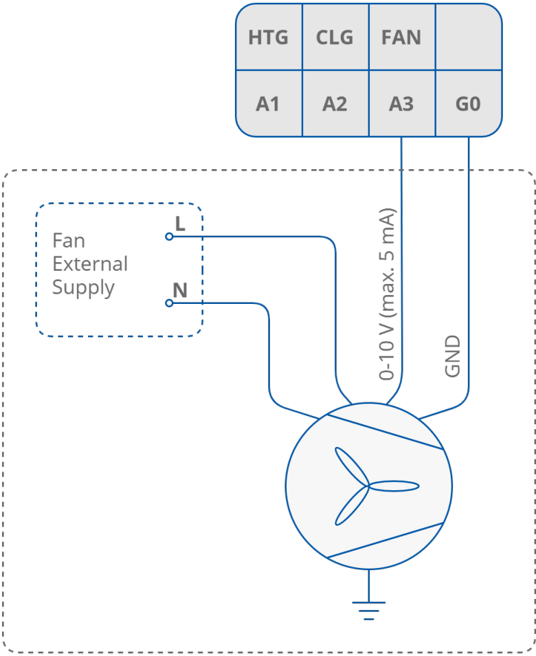
Figure 15. Connection of analog fan control
