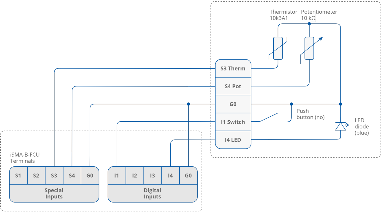
Figure 17. Connection diagram of the iSMA-B-FCU controller
