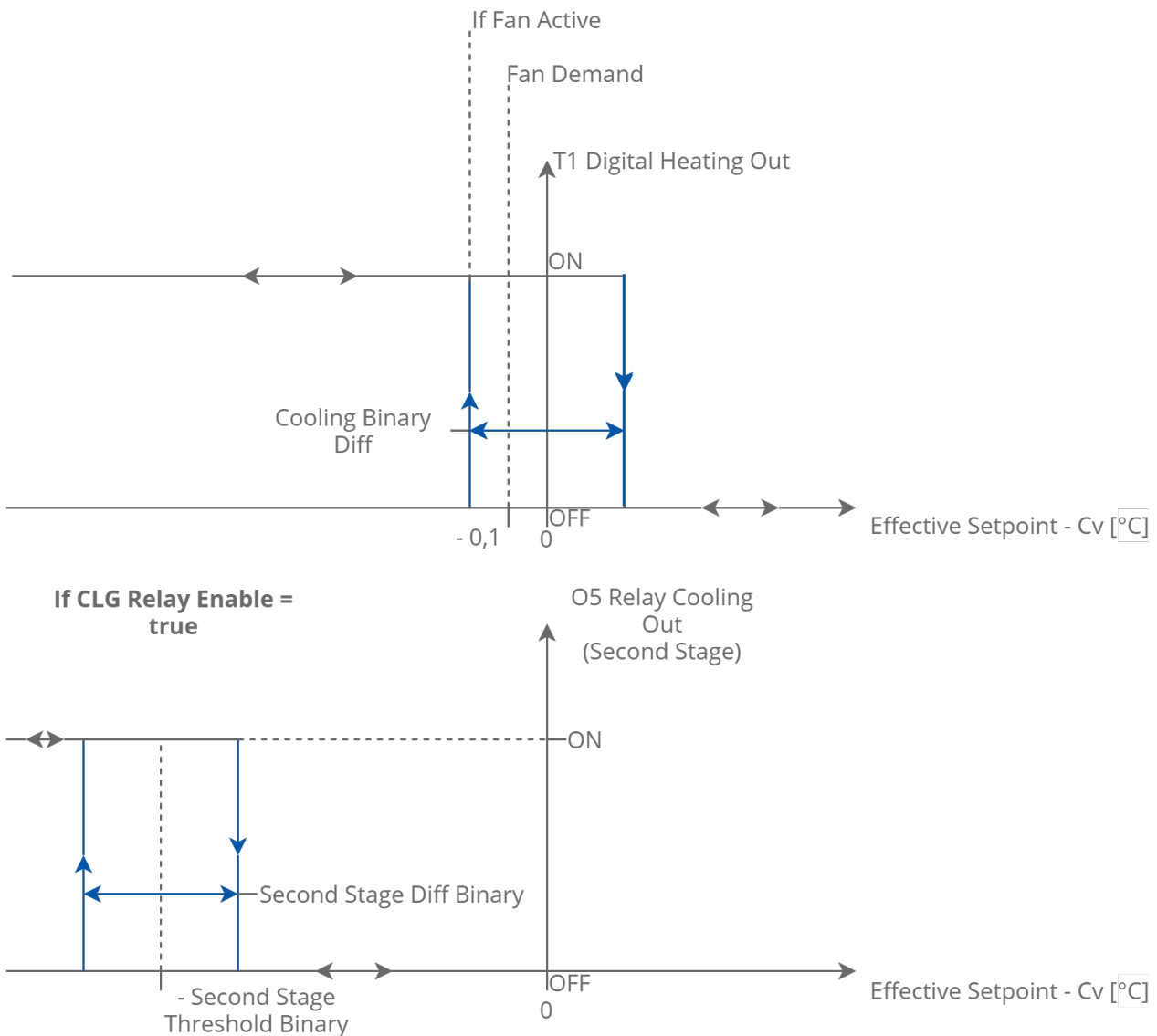
Figure 44. 2-stage cooling digital control mode
