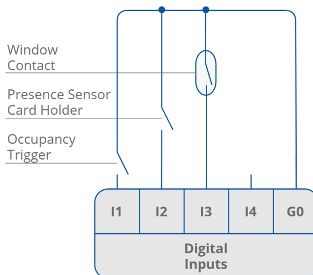
Figure 8. Digital inputs connection
