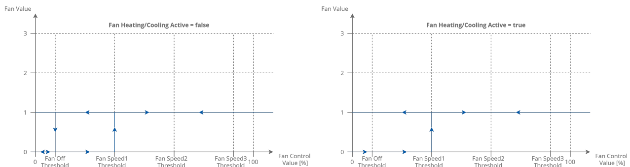
Figure 51. Fan 1-speed type control algorithm
